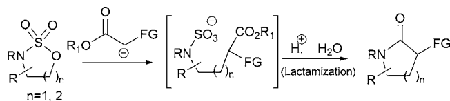
Scheme 2. Pyrrolidinones and Piperidinones via 1,2- or 1,3-Cyclic Sulfamides and Enolates
