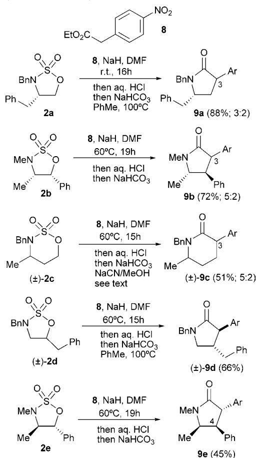
Scheme 5. Aryl-Substituted Enolates as Nucleophiles: Synthesis of \alpha -Arylated Lactams (Ar = 4-NO 2 C 6 H 4 )
