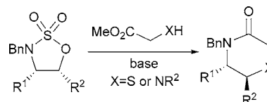
Scheme 1. Piperazinones and Thiomorpholinones from 1,2-Cyclic Sulfamidates
