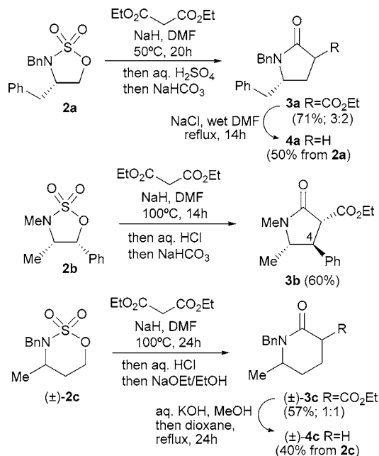
Scheme 3. Malonate as an Effective Carbon Nucleophile
