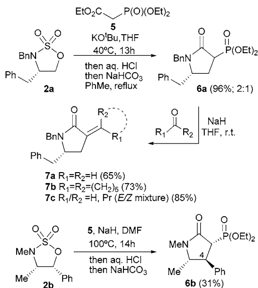
Scheme 4. Phosphonate-Stabilized Enolates and Wadsworth–Emmons Olefinations
