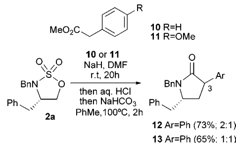
Scheme 6. Aryl-Substituted Enolates as Nucleophiles: Synthesis of \alpha -Arylated Lactams
